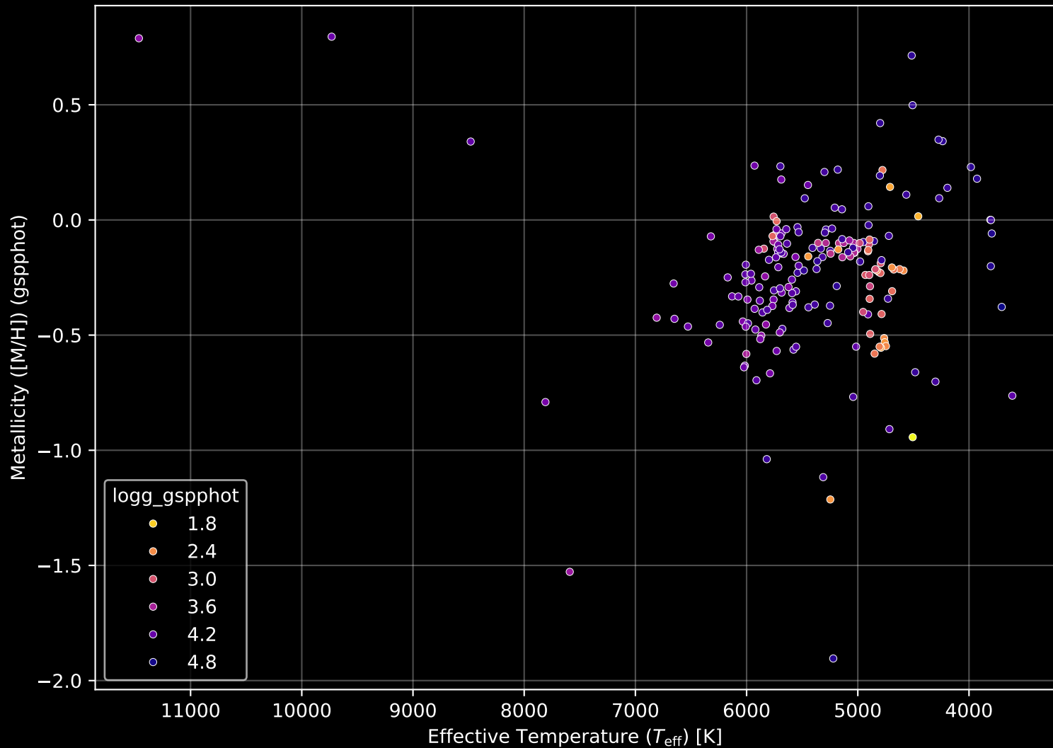
APOGEE DR17 Field: [198+38_MGA] Stellar Population Parameters (n= 194)
