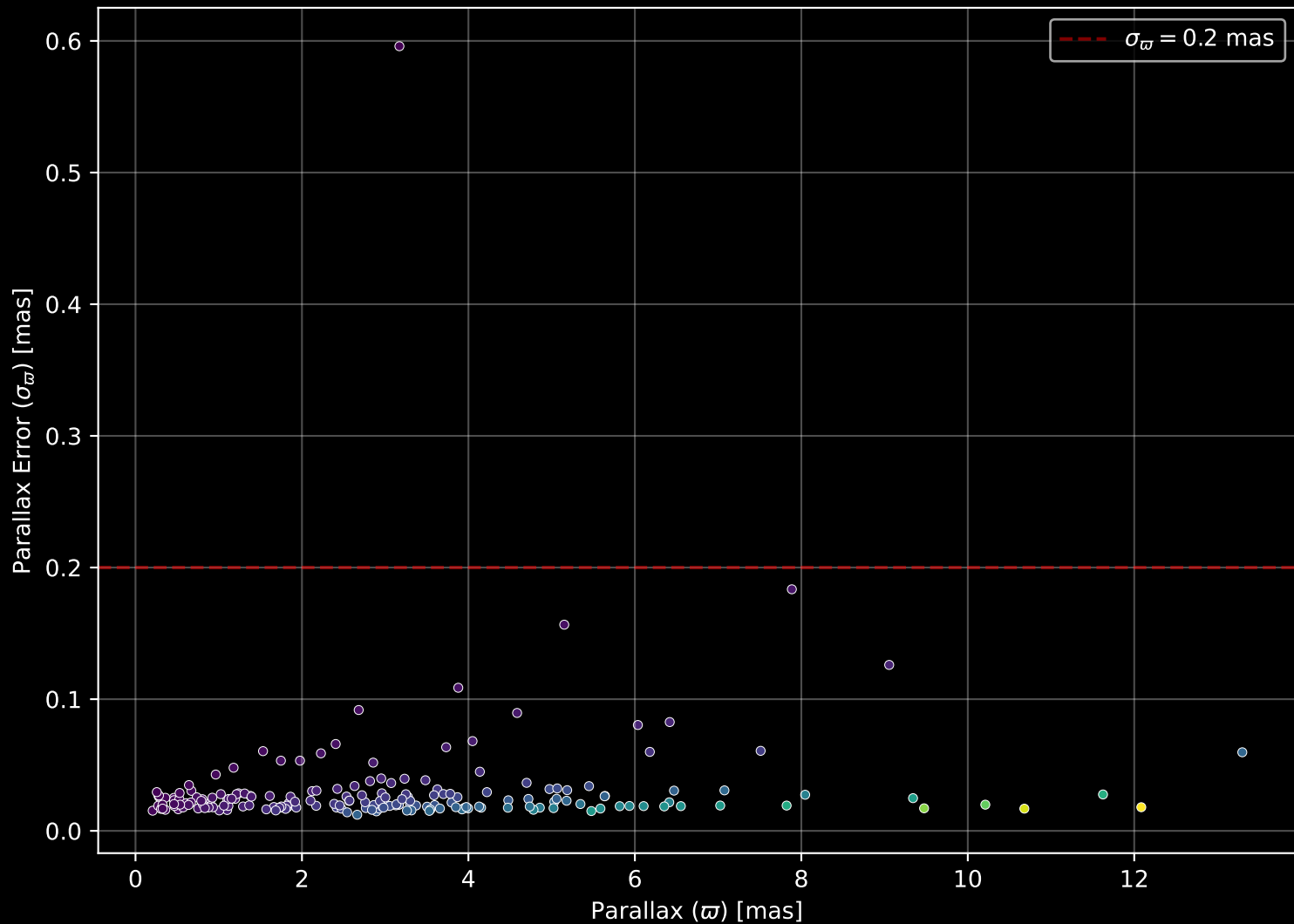
APOGEE DR17 Field: [198+38_MGA] Parallax Quality (n= 194)
