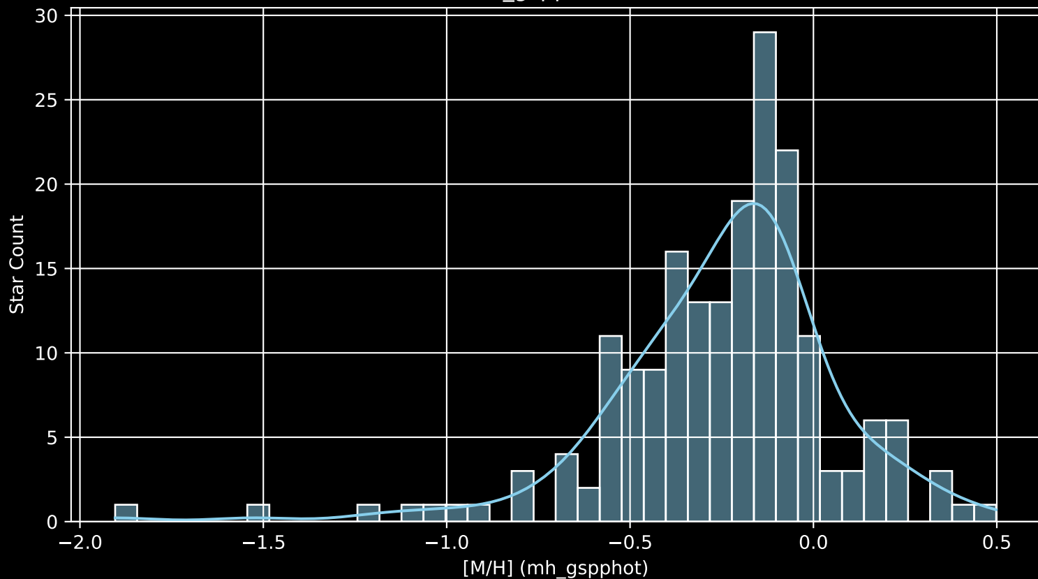
APOGEE DR17 Field: [198+38_MGA [M/H] (mh_gspphot) (n= 191)
