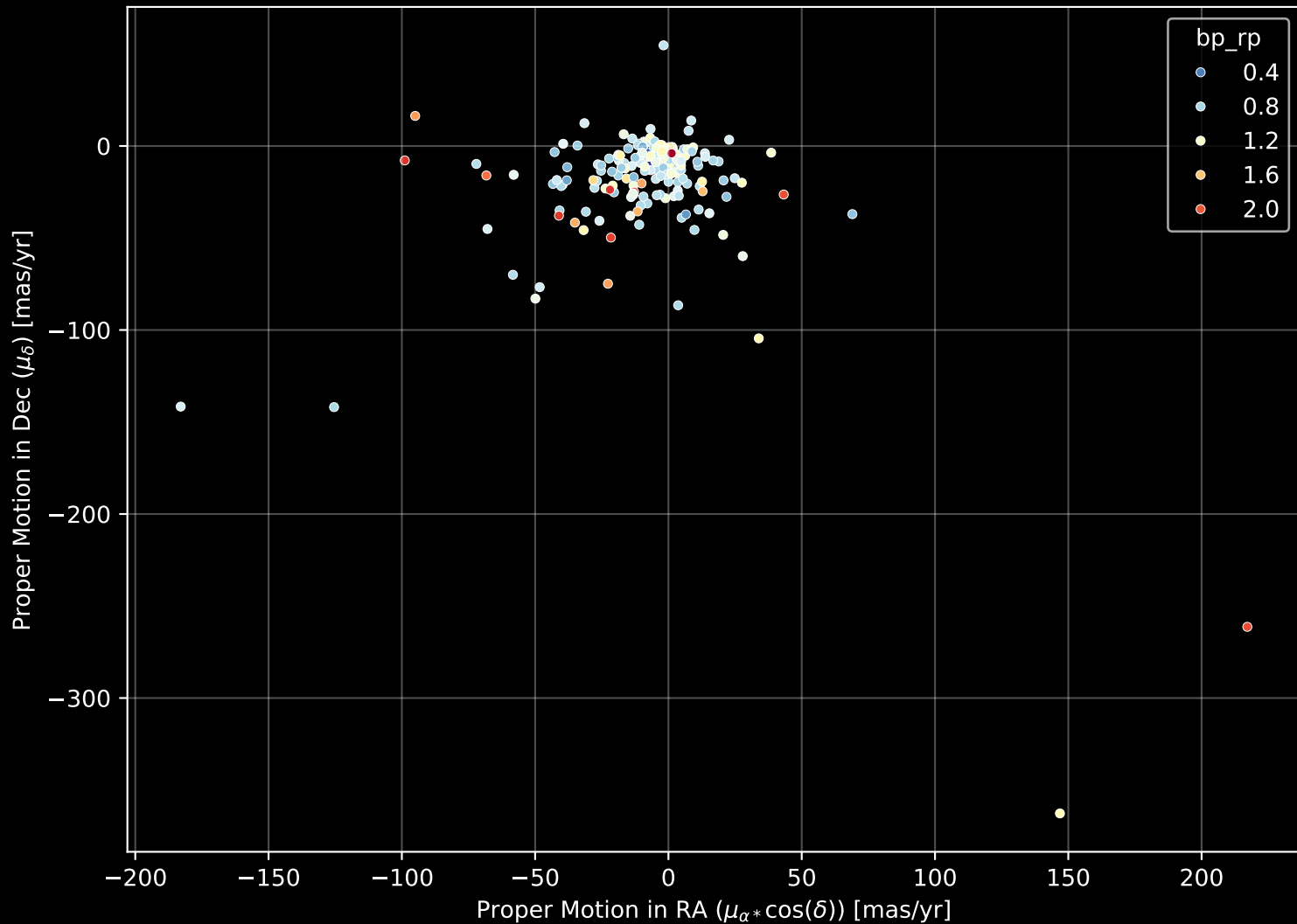
APOGEE DR17 Field: [198+38_MGA] Proper Motion Diagram (n= 194)
