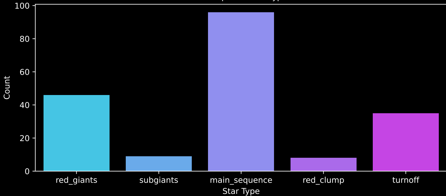
APOGEE DR17 Field: [198+38_MGA] Count plot of Star Type
