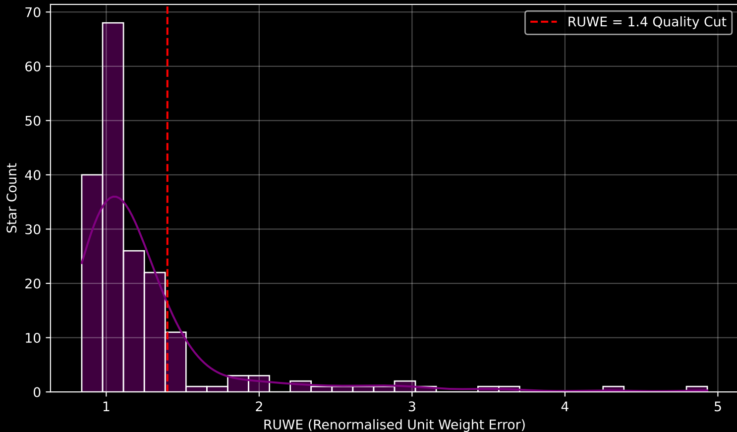
GAPOGEE DR17 Field [198+38_MGA] RUWE Distribution (n= 188)
